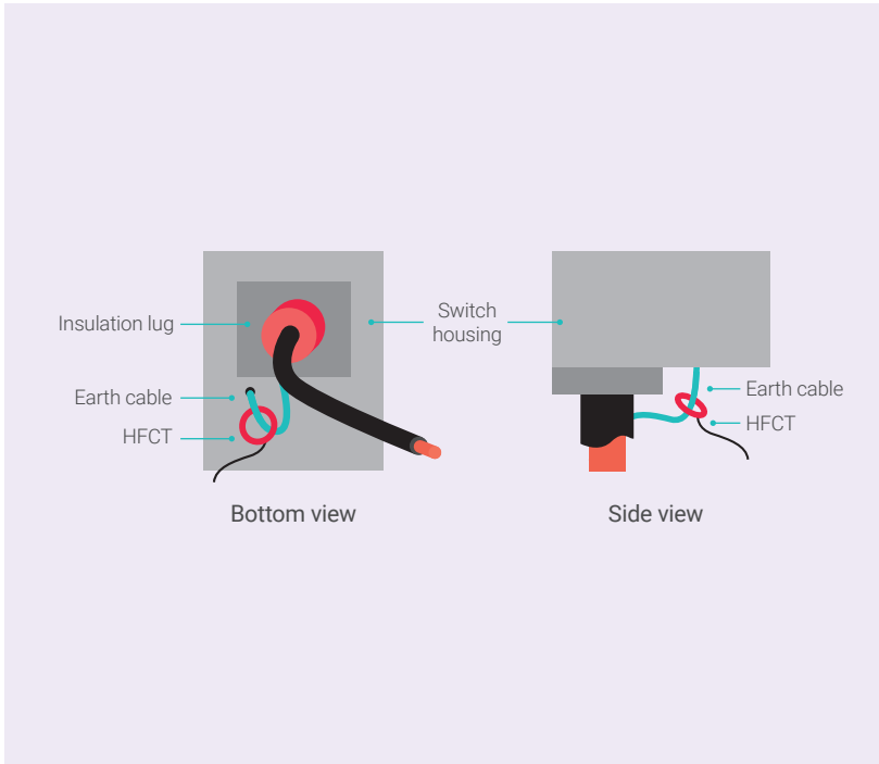
Figure 3: HFCT Connections
