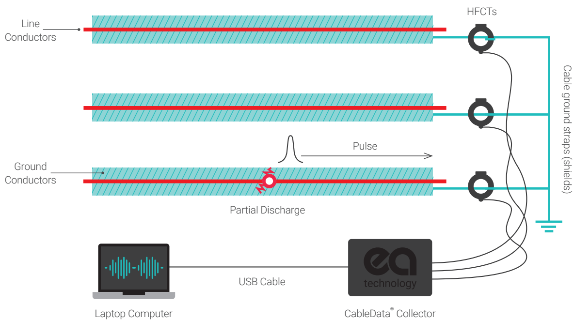
Figure 1: Setup for three phase data capture
